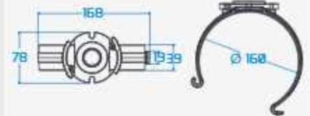
Ring-Holder for fire extinguisher of 6 Kg.
